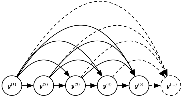
Figure 10.7: Fully connected graphical model for a sequence y^{(1)}, y^{(2)}, \dots, y^{(t)}, \dots . Every past observation y^{(i)} may influence the conditional distribution of some y^{(t)} (for t > i ), given the previous values. Parametrizing the graphical model directly according to this graph (as in equation 10.6) might be very inefficient, with an ever growing number of inputs and parameters for each element of the sequence. RNNs obtain the same full connectivity but efficient parametrization, as illustrated in figure 10.8.
