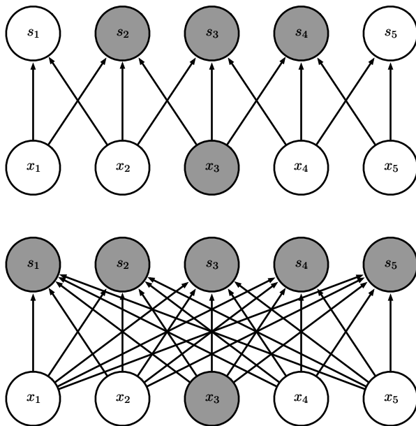
Figure 9.2: Sparse connectivity, viewed from below. We highlight one input unit, x_3 , and highlight the output units in s that are affected by this unit. (Top)When s is formed by convolution with a kernel of width 3, only three outputs are affected by x . (Bottom)When s is formed by matrix multiplication, connectivity is no longer sparse, so all the outputs are affected by x_3 .
