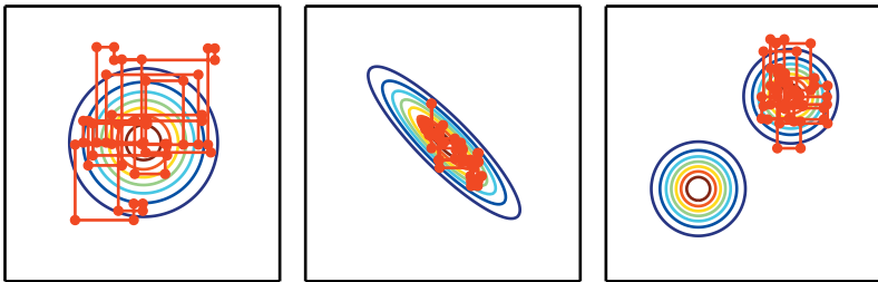
Figure 17.1: Paths followed by Gibbs sampling for three distributions, with the Markov chain initialized at the mode in both cases. ( Left ) A multivariate normal distribution with two independent variables. Gibbs sampling mixes well because the variables are independent. ( Center ) A multivariate normal distribution with highly correlated variables. The correlation between variables makes it difficult for the Markov chain to mix. Because the update for each variable must be conditioned on the other variable, the correlation reduces the rate at which the Markov chain can move away from the starting point. ( Right ) A mixture of Gaussians with widely separated modes that are not axis aligned. Gibbs sampling mixes very slowly because it is difficult to change modes while altering only one variable at a time.
