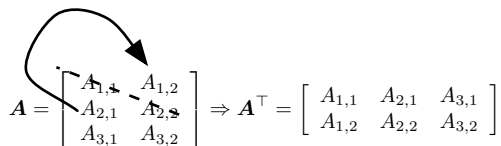
Figure 2.1: The transpose of the matrix can be thought of as a mirror image across the main diagonal.
