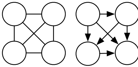
Figure 16.10: Examples of complete graphs, which can describe any probability distribution. Here we show examples with four random variables. ( Left ) The complete undirected graph. In the undirected case, the complete graph is unique. ( Right ) A complete directed graph. In the directed case, there is not a unique complete graph. We choose an ordering of the variables and draw an arc from each variable to every variable that comes after it in the ordering. There are thus a factorial number of complete graphs for every set of random variables. In this example, we order the variables from left to right, top to bottom.
