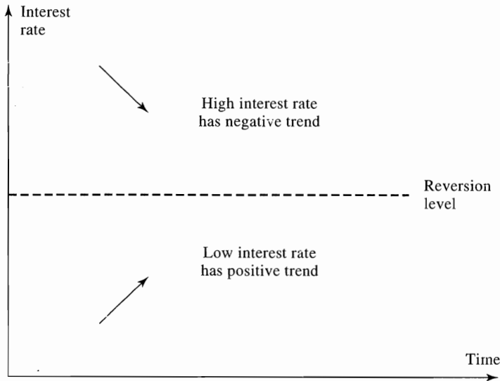
Figure 30.1 Mean reversion.
