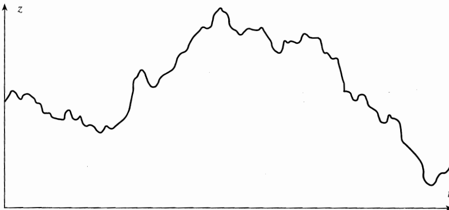
Smaller value of \Delta t
