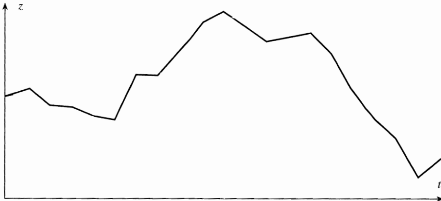
Relatively large value of \Delta t
