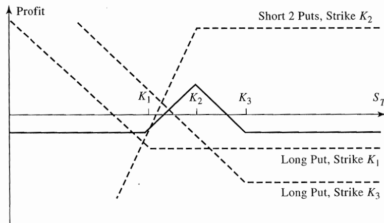
Figure 11.7 Profit from butterfly spread using put options.
