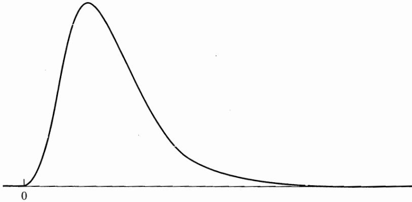
Figure 14.1 Lognormal distribution.
