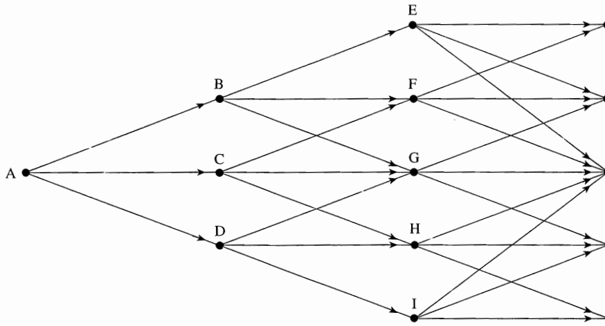
Figure 30.8 Tree for R^* in Hull–White model (first stage).
