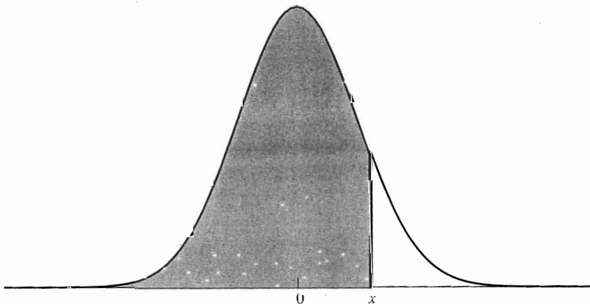
Figure 14.3 Shaded area represents N(x) .
