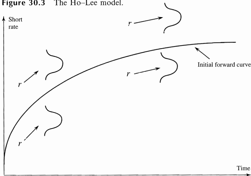
Figure 30.3 The Ho–Lee model.
