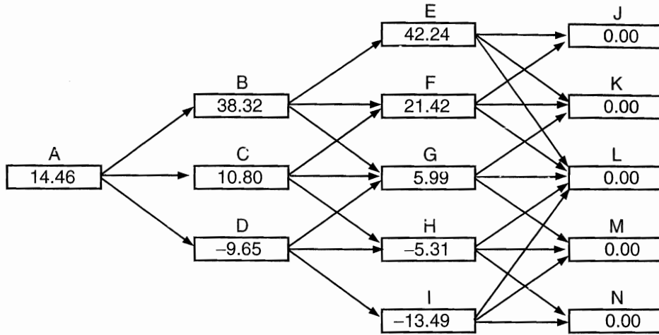
Figure 34.2 Valuation of base project with no embedded options: p_u , p_m , and p_d are the probabilities of “up”, “middle”, and “down” movements from a node.
