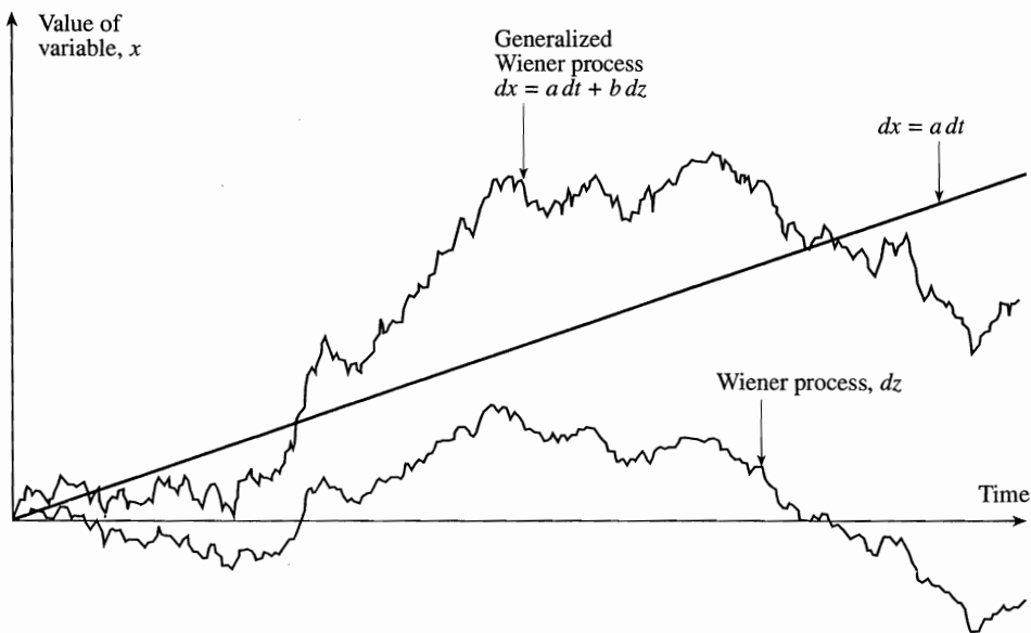
Figure 13.2 Generalized Wiener process with a = 0.3 and b = 1.5 .
