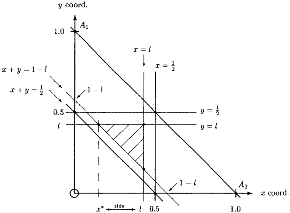
Figure D.5: Broken Stick Problem, F_L(l) = P(L \leq l) , Case: \frac{1}{3} \leq l \leq 0.5
