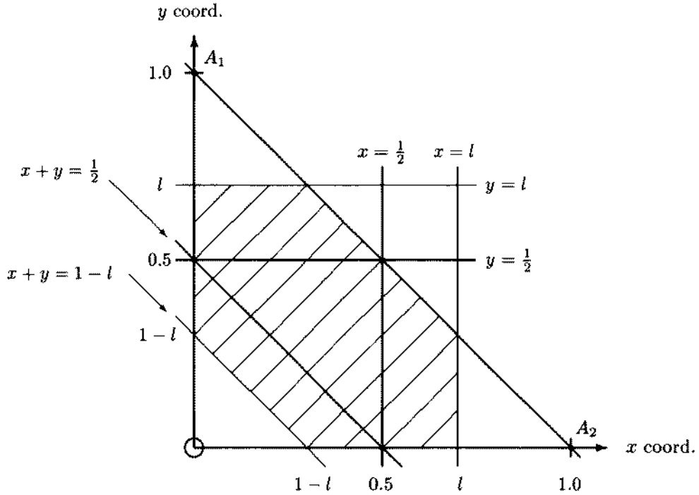
Figure D.4: Broken Stick Problem, F_L(l) = P(L \leq l) , Case: 0.5 \leq l \leq 1
